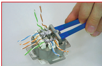
Folien der Aderpaare bündig zu den LSA-Leisten kürzen. / Cut foil over pairs that way, that it is as close to LSA-connection module as possible.
