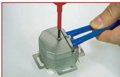
Schirmhaube festschrauben. / Fix Shield-Cover with screw.
