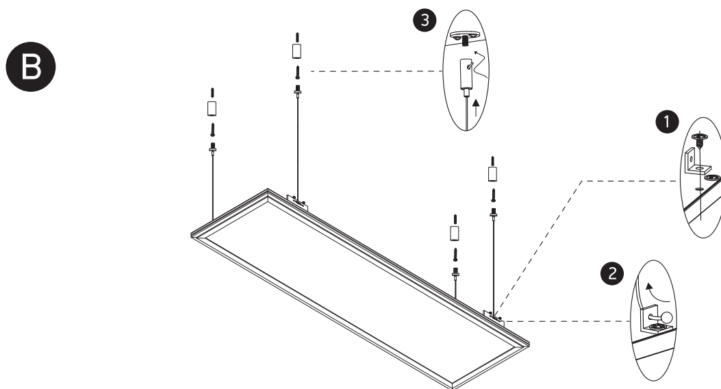
Ceiling mount suspended applications using optional kit 050017.
