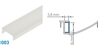
LIAB001003 PMMA Abdeckung LB Flach Opal PMMA cover LB flat milky
