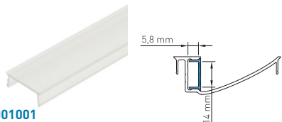
LIAB001001 PMMA Abdeckung LB Flach Transparent PMMA cover LB flat transparent
