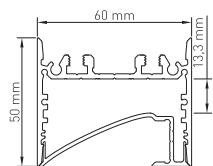
Aluminium Profil SLW glatt im SLR Profil Aluminium profile SLW smooth in SLR profile
