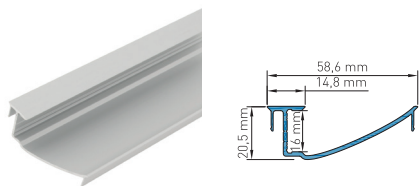
LIAP003100 Aluminium Profil SLW glatt Aluminium profile SLW smooth
