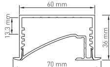
Aluminium Profil SLW glatt im SLI Profil Aluminium profile SLW smooth in SLI profile
