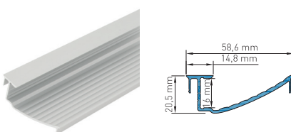
LIAP003200 Aluminium Profil SLW geriffelt Aluminium profile SLW rippled
