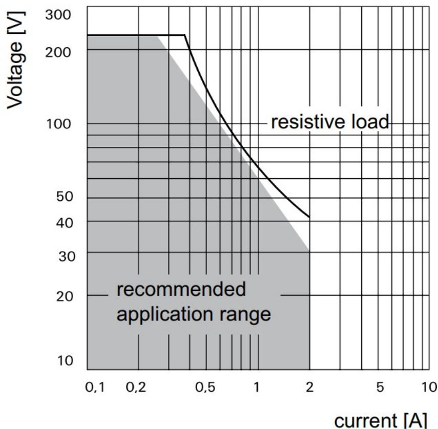
Load curve of signal relays (AC/DC)
